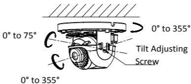
Figure 2-6 Type II Camera 3-Axis Adjustment
